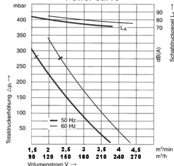
Power curve
